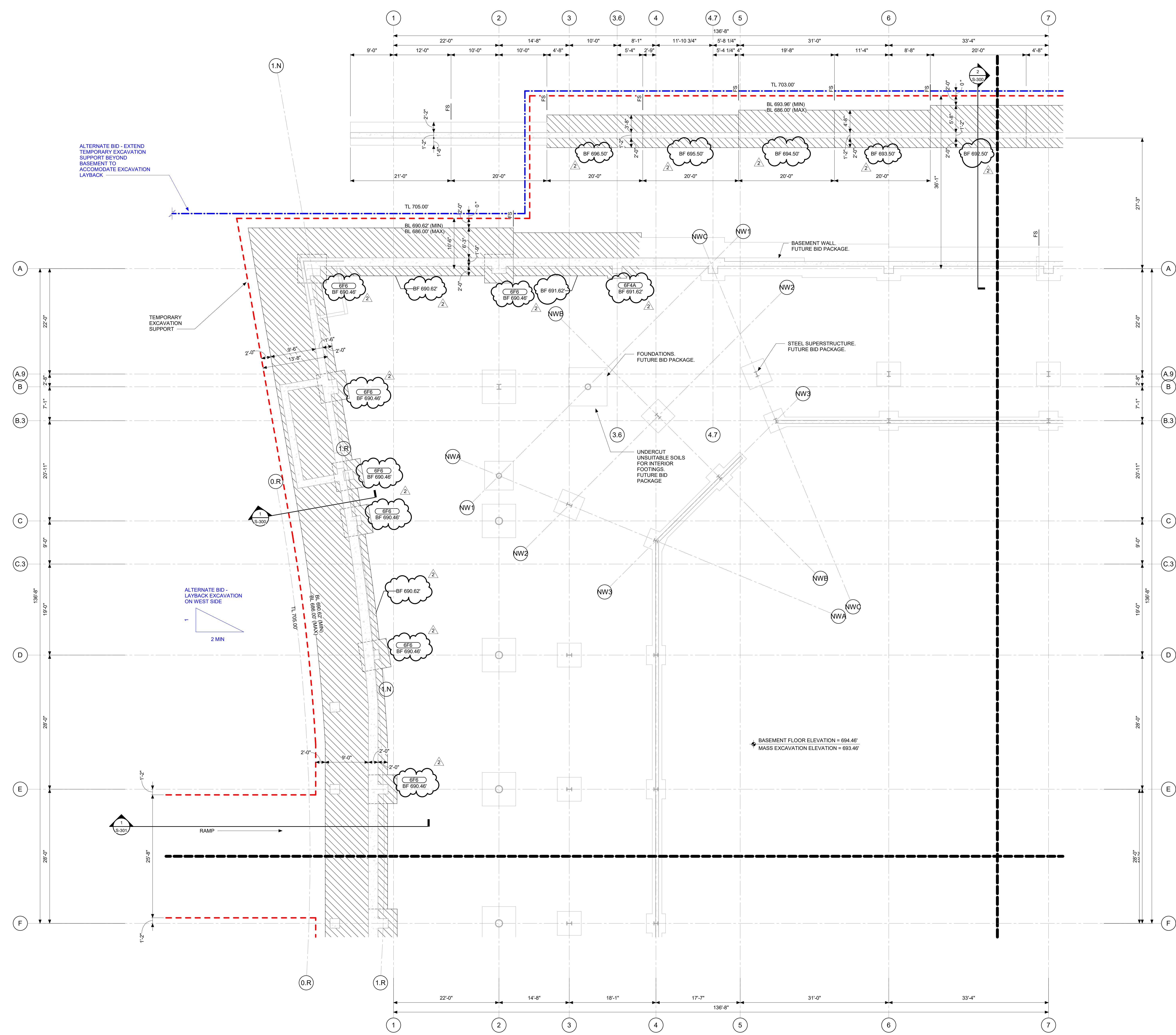
1 EXCAVATION PLAN - UNIT A SCALE: 1/8" = 1'-0"
